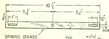
DIMENSIONS ARE FOR A 3" FORM.
