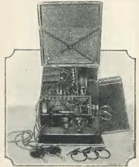
The prize-winning portable receiver opened and ready for operation. Note the headphones and the inductors in the foreground.
