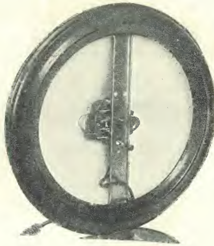
Left: The back of the cone speaker, with the silk cover removed to show the position of the drive-unit on the upright section of the frame. Right: The front of the same speaker. Illustrations courtesy Bondette Mfg. Co.
