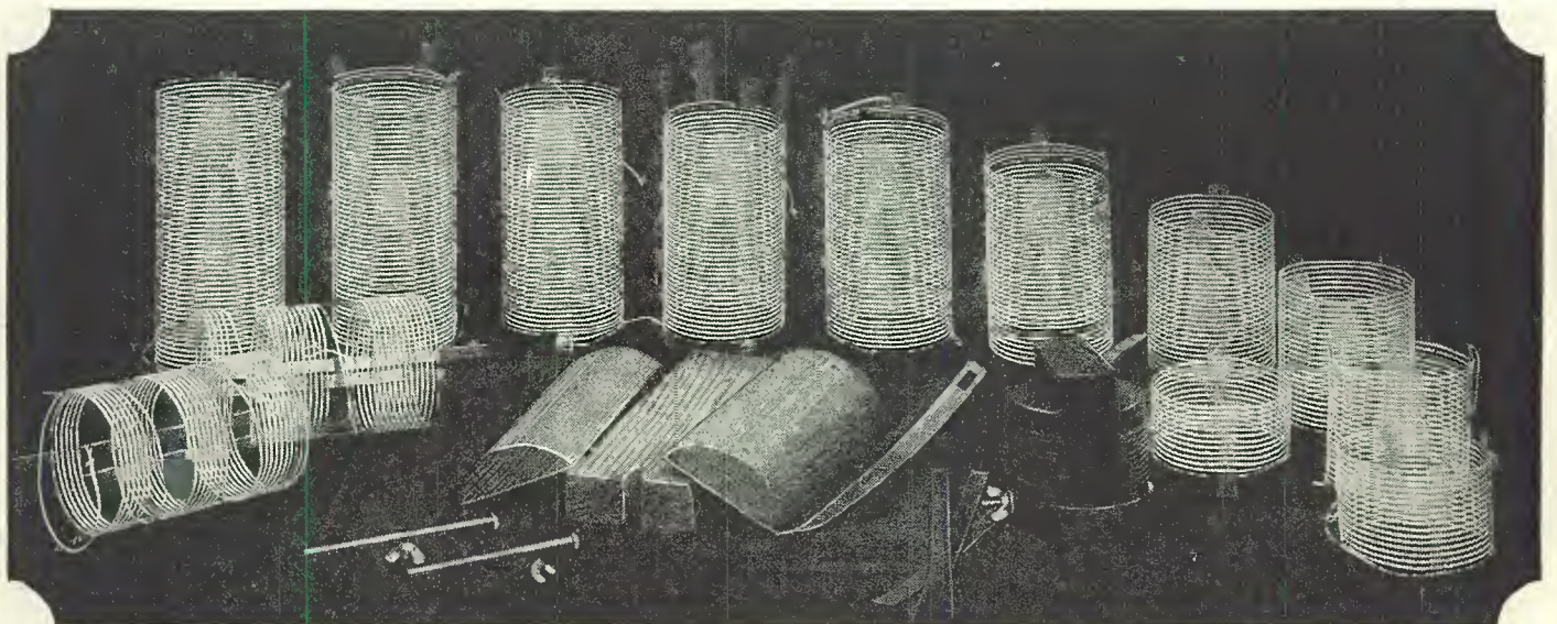
A group of extremely low-loss coils, wound by the author, and two of the coil forms which he has developed. The large coils cover the broad-
