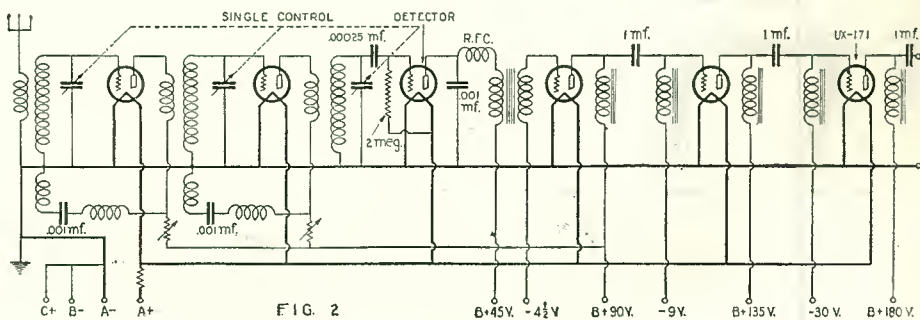
FIG. 2 The complete circuit diagram of the author's receiver.
