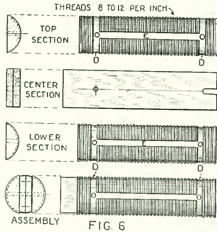
Additional details for the construction of the wooden form on which the coils are wound.
