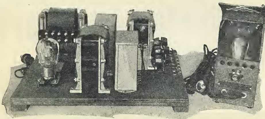
At the left is a 350-milliamperer "A, B and C" unit for 201-A tubes in series; and at the right an 85-milliamperer unit for 199-type tubes in series.
