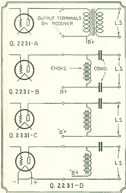
The various types of output filter devices shown here are used to protect the loud speaker from being damaged by heavy currents. They are fully explained in the text.
