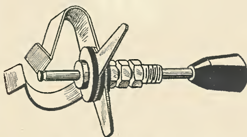
The little plunger-rod of this filament switch can be removed completely from the sleeve in which it fits. Illustration courtesy Owen, Berlin.
