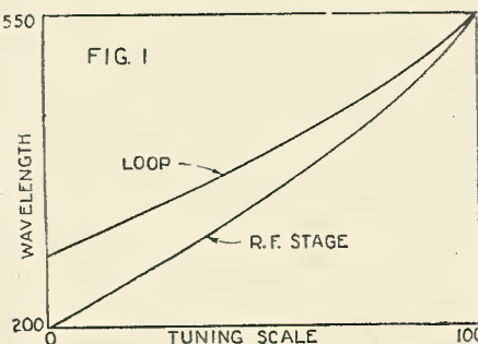
These two curves show how the tuning of the Strobodyne is off at the lower wavelengths without a second shunt condenser.
