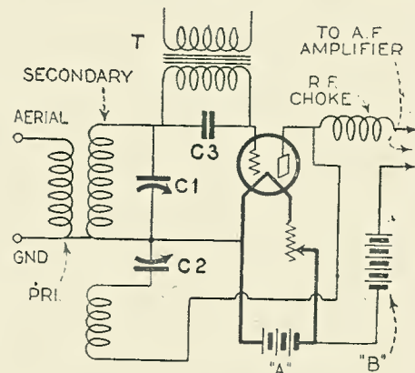
Fig. 1. This shows in schematic form the detector section of the RADIO NEWS short-wave broadcast receiver.
