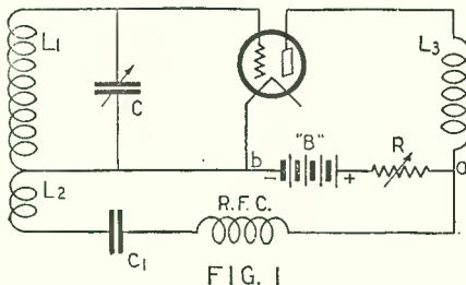
FIG. 1 The fundamental circuit diagram of the R.F. stage which is the heart of the set.
