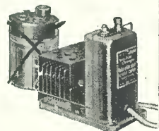
How the Kuprox Replacement Unit replaces the acid jar on trickle chargers.
