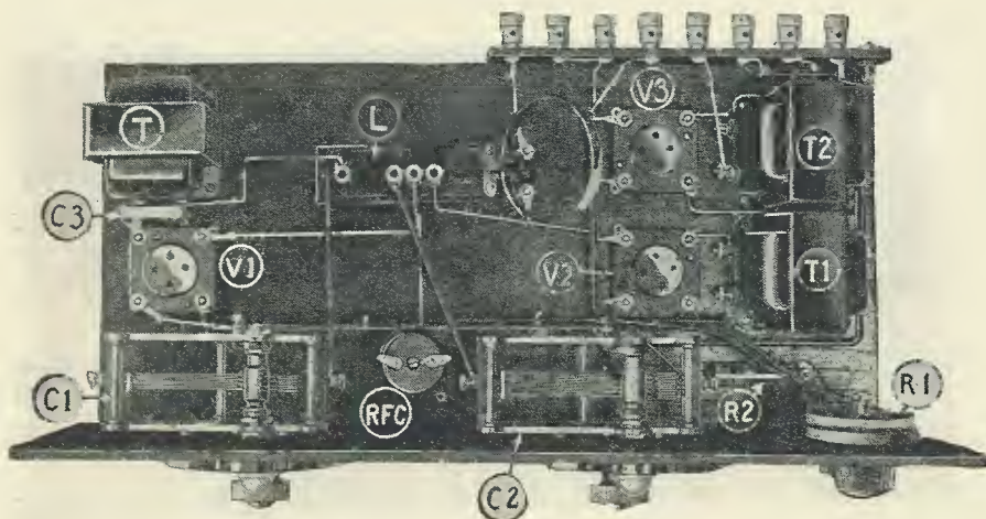
Top view of the complete three-tube short-wave receiver of which will be described in detail in next month's RADIO NEWS. C1, tuning condenser; C2, regeneration control; L, plug-in coil base; T, grid choke; C3, grid condenser; R.F.C., R.F. choke; T1, T2, A.F. transformers; R1, R2, filament resistors; V1, V2, V3, tube sockets.
