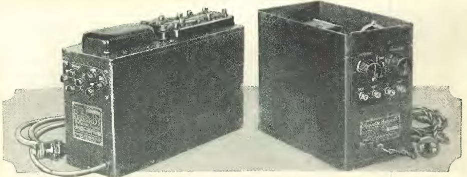
The "B" socket-power unit at the left is of the chemical type; and the other uses a rectifier tube. Photo by courtesy of Faustel Products Co. and Grigsby-Gruncow-Hinds Co.
