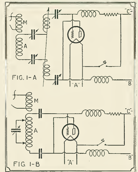
Two methods of connecting the Moduloscope in a transmitting circuit.
