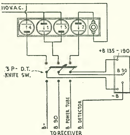
Fig. 1. Wiring diagram of the complete "B" charger unit.
