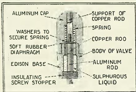
The internal construction of the "Sulfootron" rectifying tube, showing the location of the various parts, as explained in the text.
